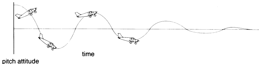
Figure 14. Positive Dynamic Pitch Stability
