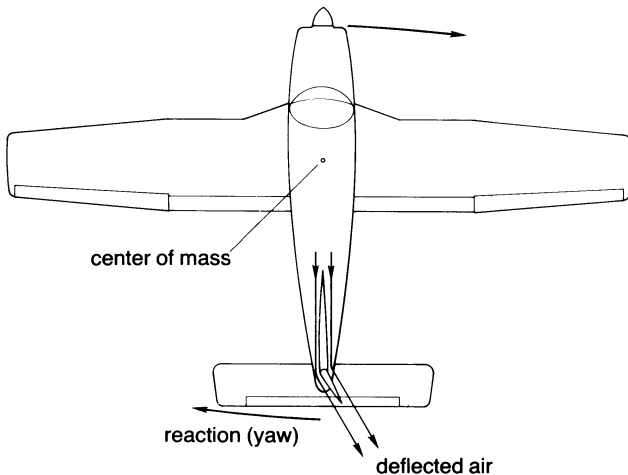
Figure 15. Deflection of Air by the Rudder
