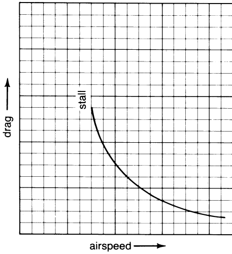
Figure 11. Induced Drag versus Airspeed
