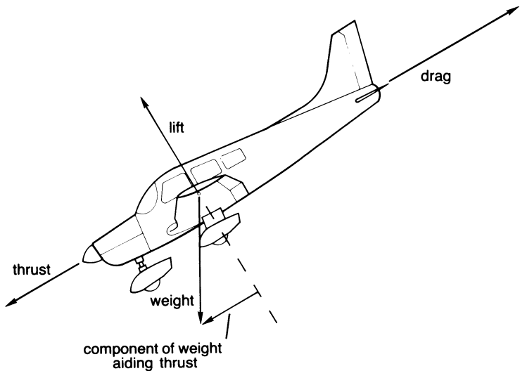
Figure 17. Steady Descent: Drag = Thrust + Component Of Weight Aiding Thrust
