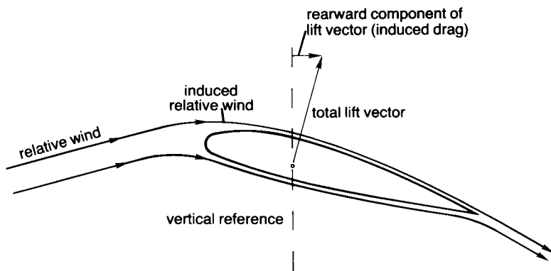
Figure 10. Induced Drag Due To Induced Relative Wind
